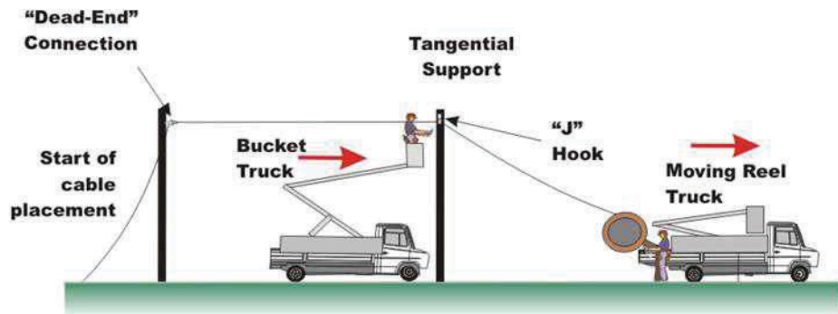
Figure 38- Moving Reel ADSS Cable Placing Method
