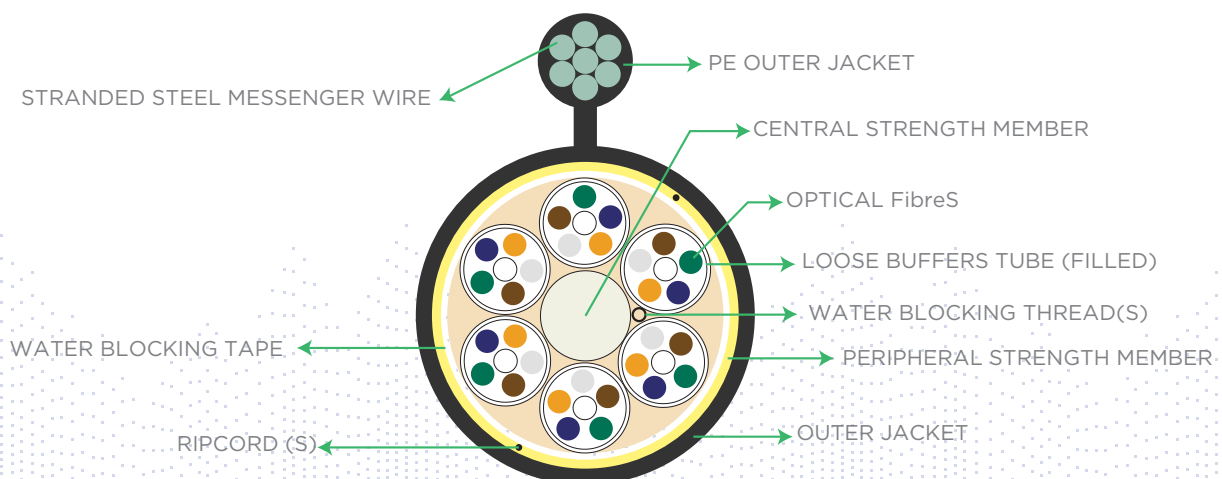
Figure 2- STL Loose Tube Figure-Eight weOight apt insttaliatcional Cable for Aerial Applications
