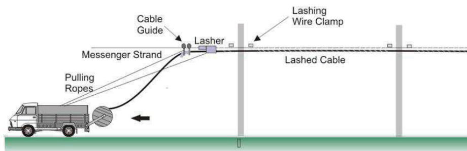
Figure 11– Schematic Drawing of the Moving Reel (Drive-Off Method) to Place Aerial Cable
