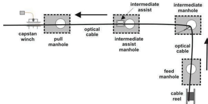
Figure 4– Schematic Showing Intermediate-Assist Manhole
