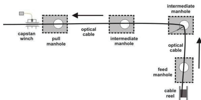
Figure 1– Schematic Showing Different Types of Manholes
