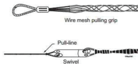
Figure 7– Basket Grip and Ball-Bearing Swivel at Lead End of Cable
