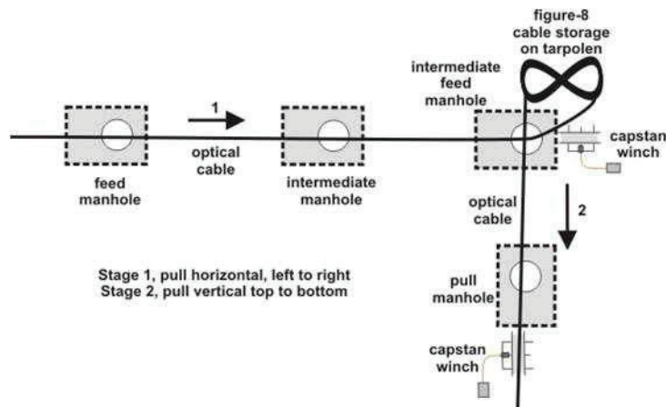
Figure 2– Schematic Showing Intermediate-Feed Manhole
