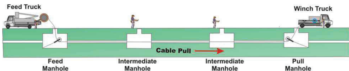
Figure 6– Cable Pulling Showing Placement Without Intermediate Assist
