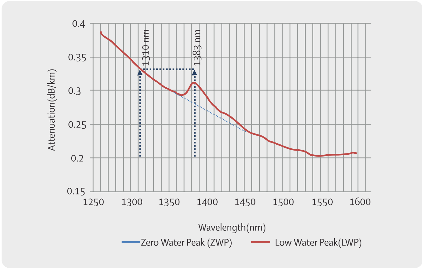
Figure 1 Typical Spectral attenuation plot of Zero and Low Water Peak fiber
