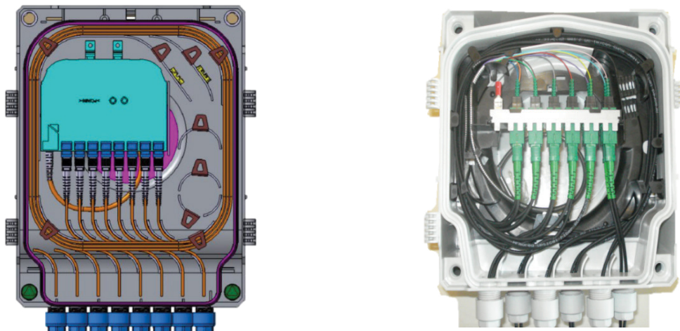
Figure 1 Distribution boxes with pre-connectorized cable
